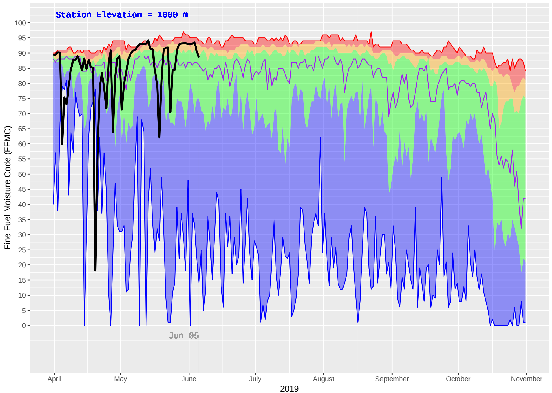
SUCCOUR CREEK (374) : Historical (1986–2018) and Current (2019) Daily Fine Fuel Moisture Code (FFMC)
