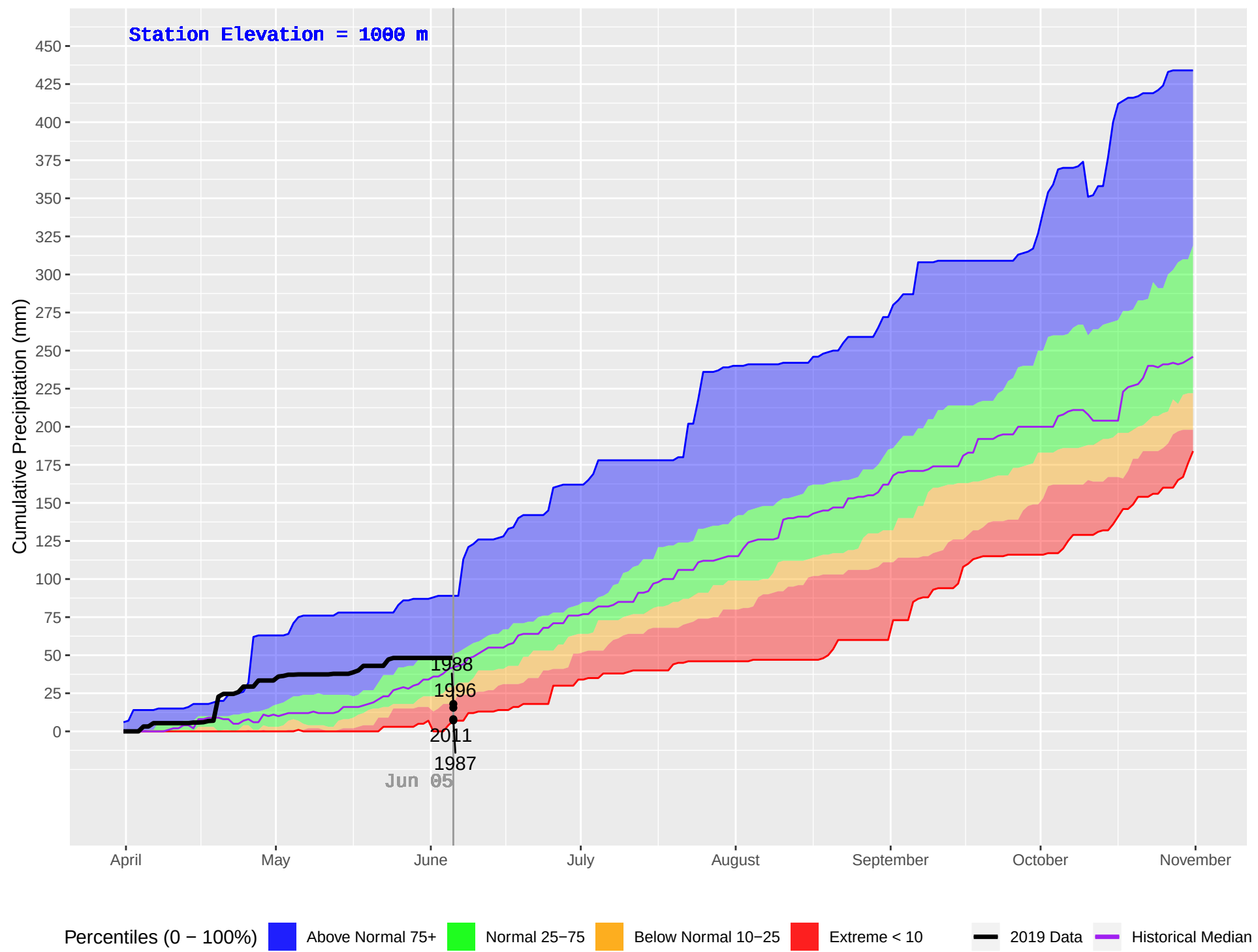
SUCCOUR CREEK (374) : Historical (1986–2018), Current (2019) Daily Cumulative Precipitation
