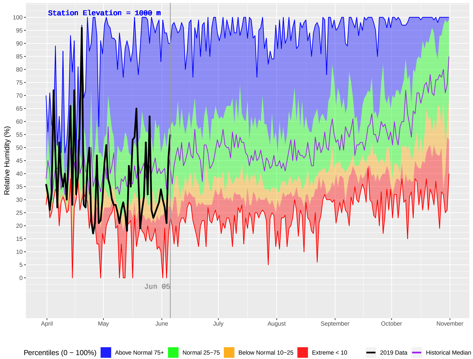
SUCCOUR CREEK (374) : Historical (1986–2018) and Current (2019) Daily Relative Humidity
