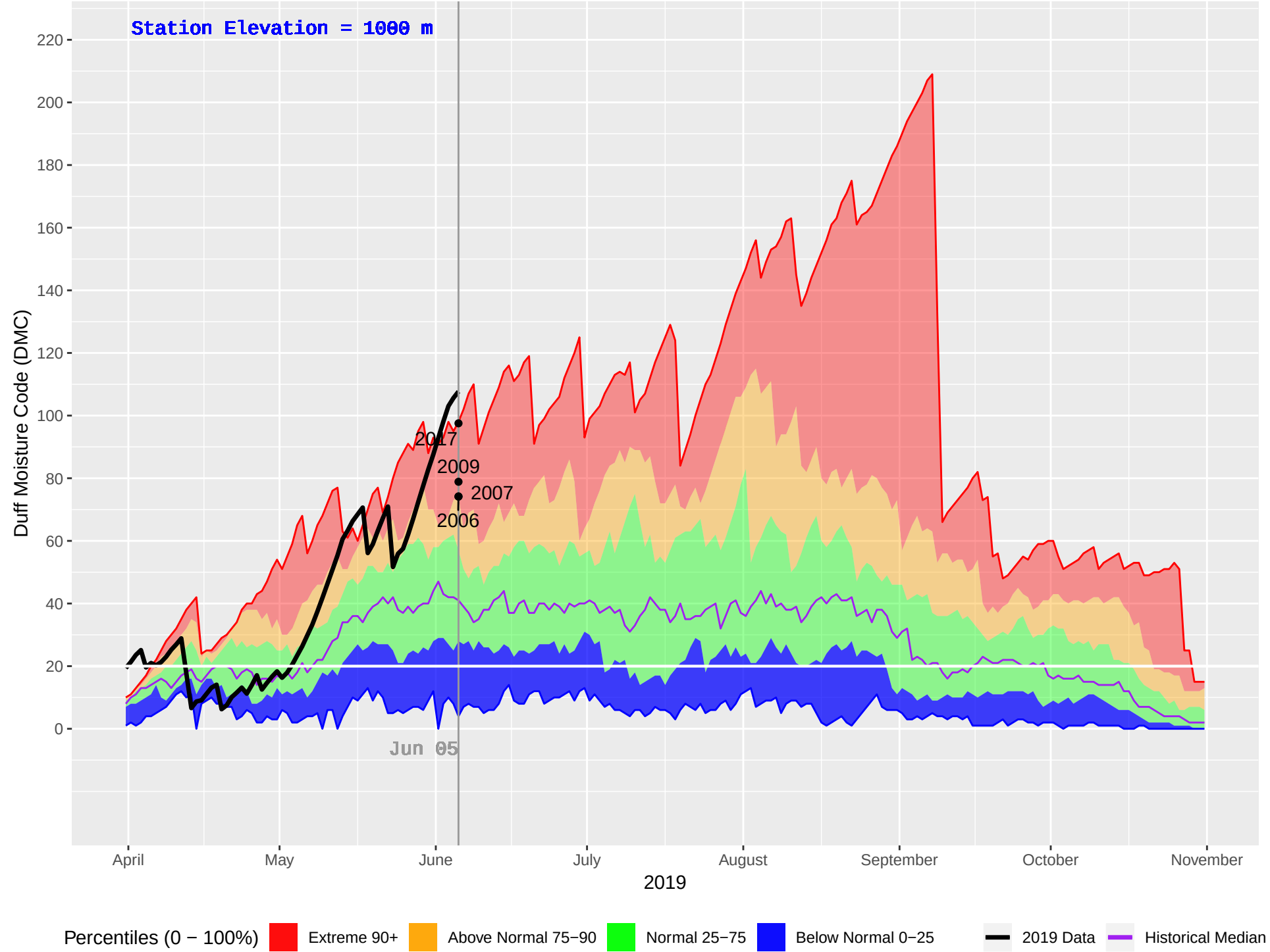
SUCCOUR CREEK (374) : Historical (1986–2018), Current (2019) Daily Duff Moisture Code (DMC)
