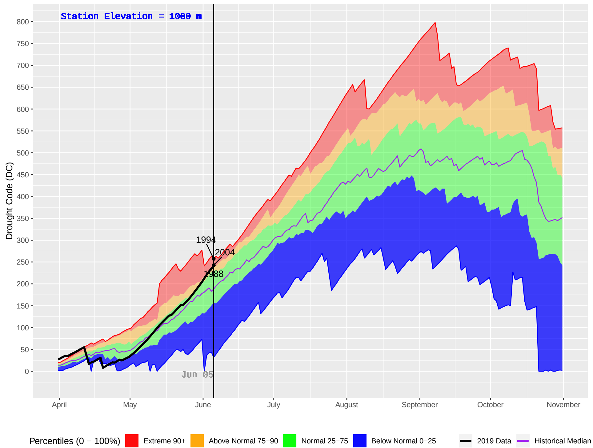
SUCCOUR CREEK (374) : Historical (1986–2018) and Current (2019) Daily Drought Code (DC)
