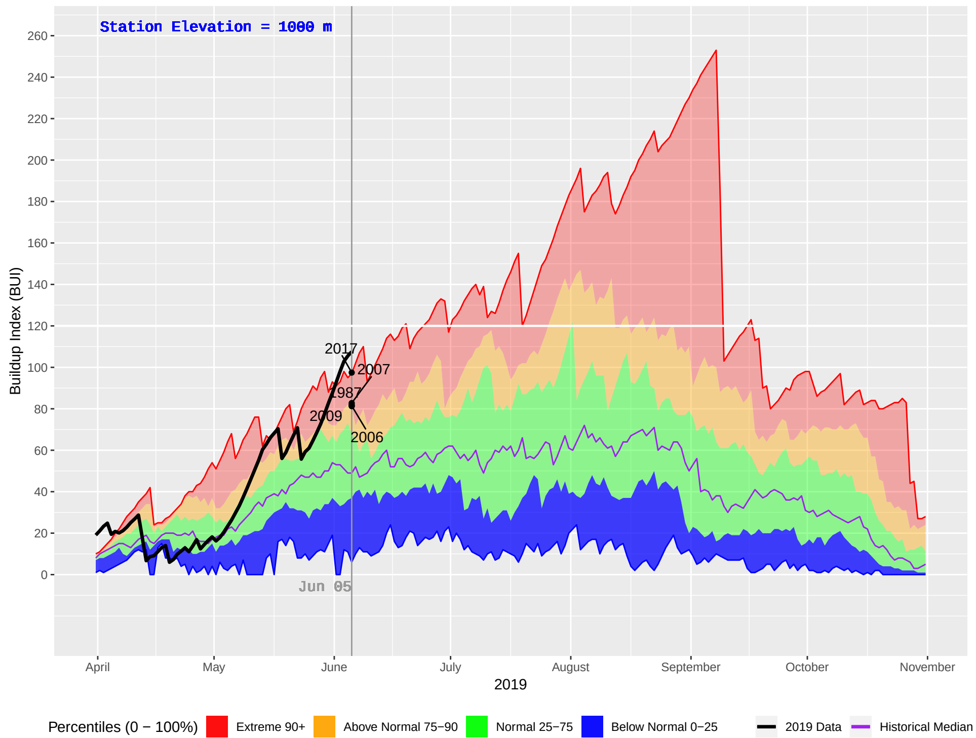
SUCCOUR CREEK (374) : Historical (1986–2018), Current (2019) Daily Buildup Index (BUI)
